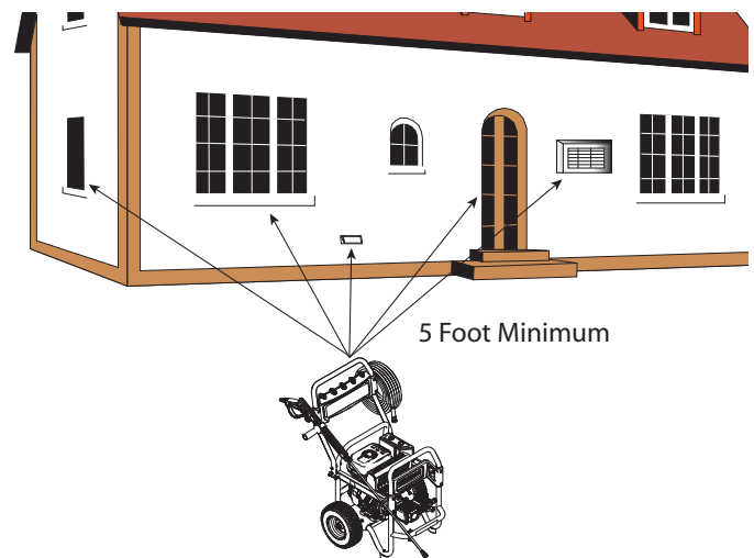
Figure 23 – Building Clearances
